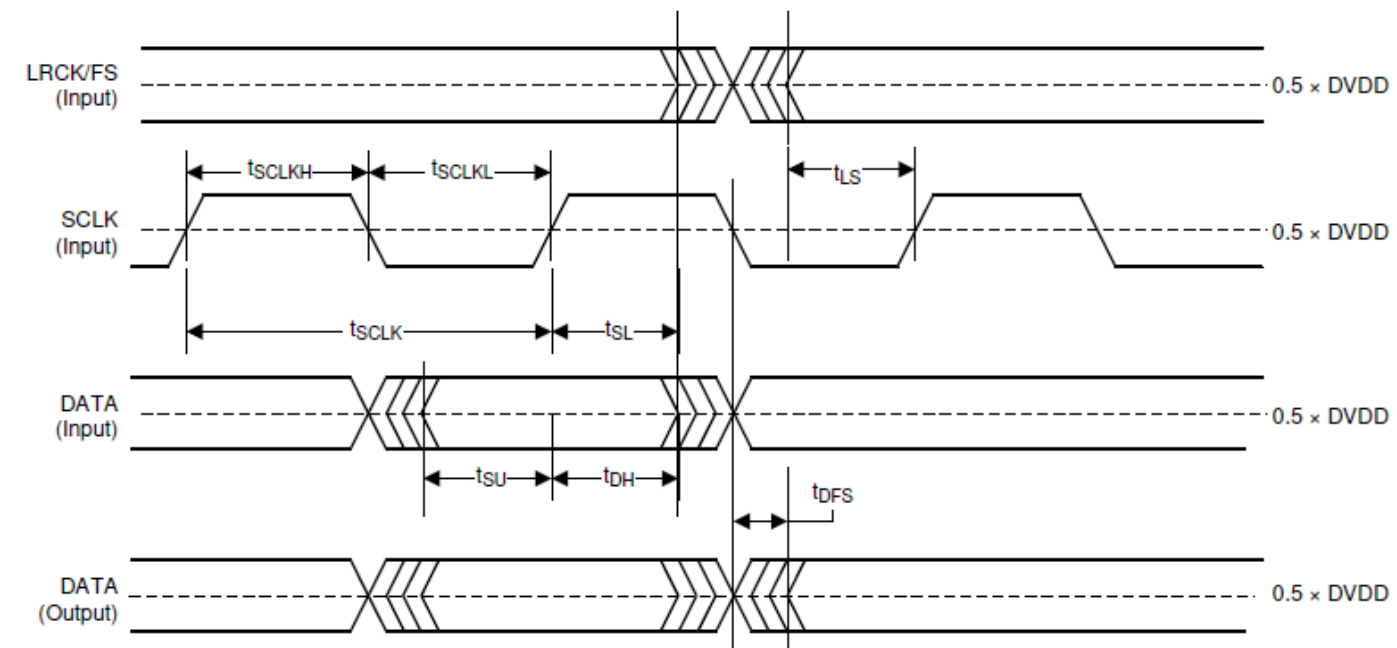
Figure 2. Serial Audio Port Timing in Slave Mode
