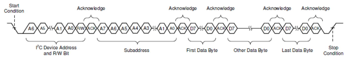
Figure 14. Sequential Write Transfer
