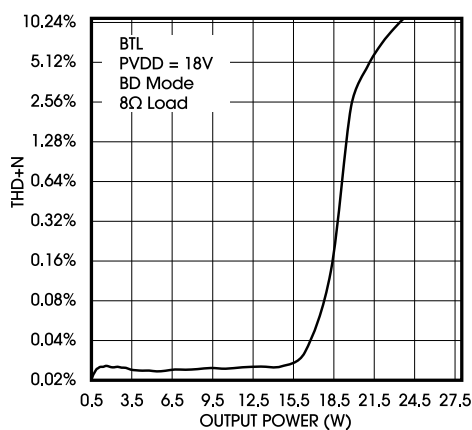
Figure 9. THD+N vs. Output Power (BTL)
