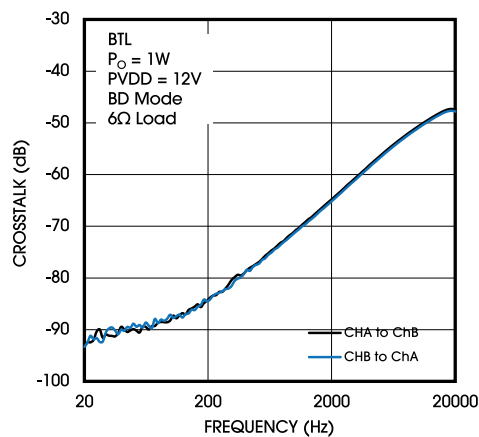
Figure 10. Crosstalk (BTL)
