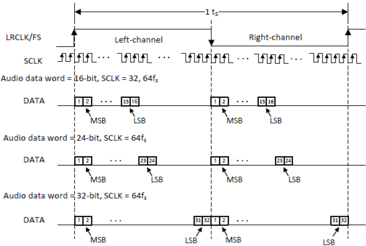
Figure 5. Left-Justified Audio Data Format
