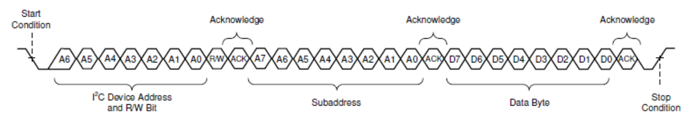
Figure 13. Random Write Transfer
