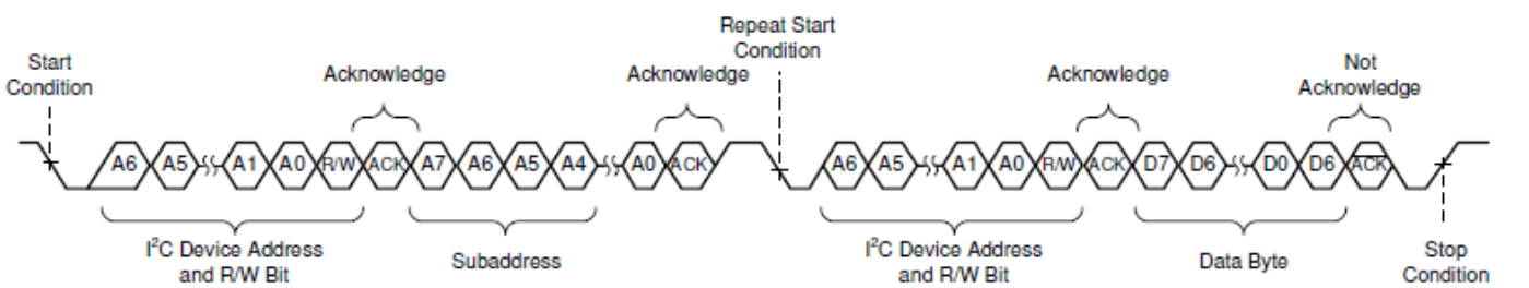
Figure 15. Random Read Transfer
