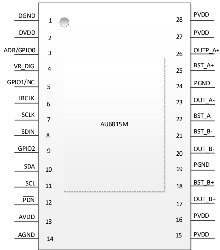
Figure 1. Pin Configuration
