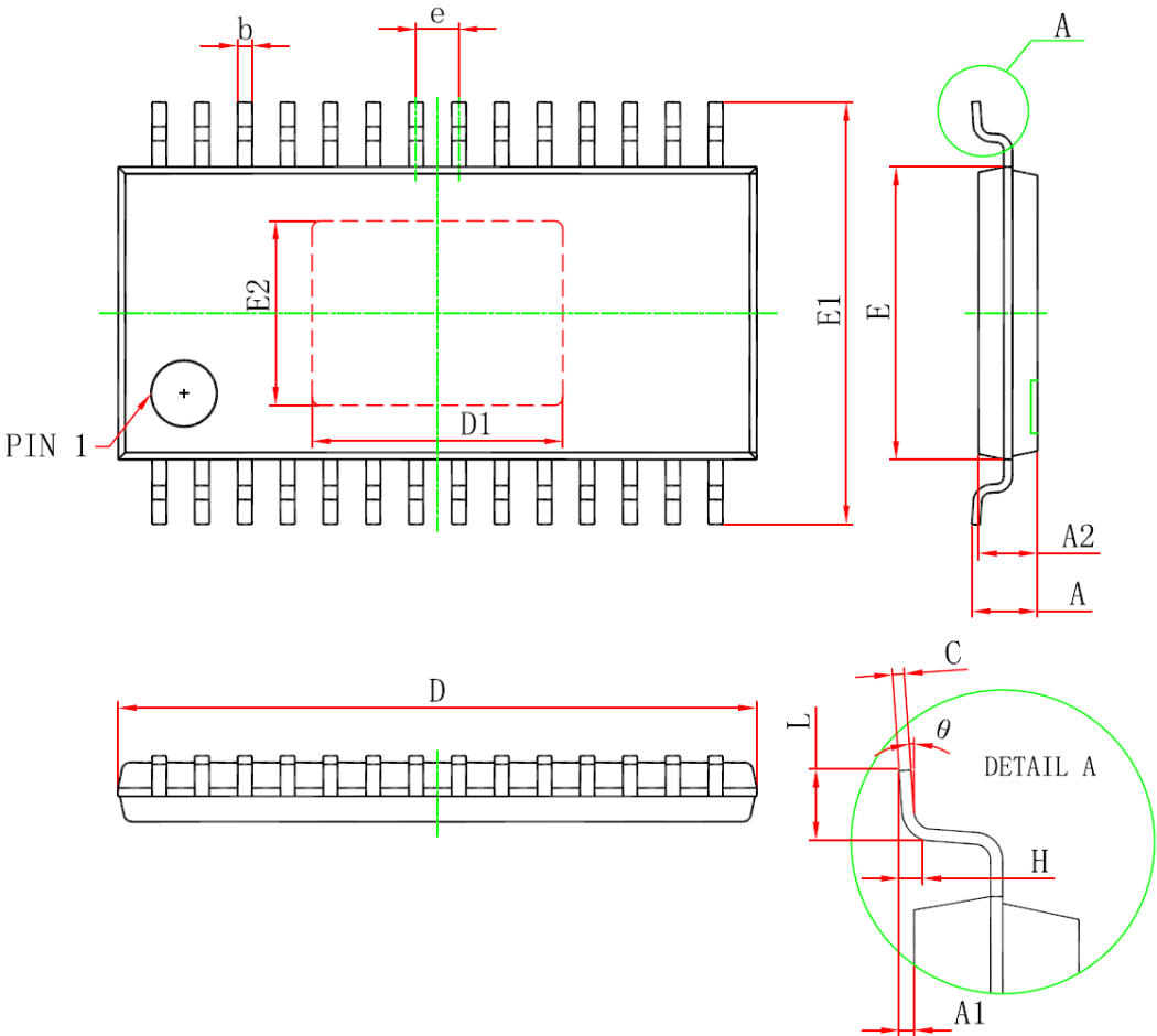
Figure 21. Package View
