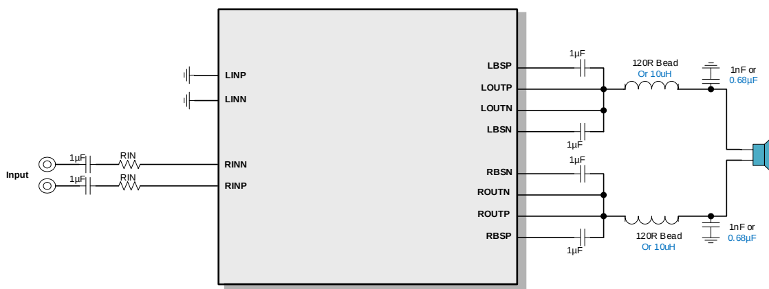
Figure 4 PBTL configuration
