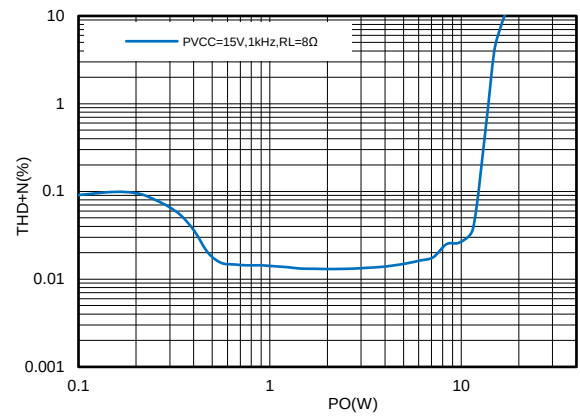
图34. 15V供电8Ω负载THD+N曲线PBTl
