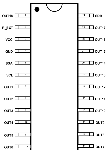
HTR3218P Top View
