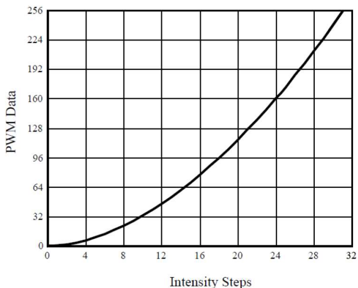
Figure 5 Gamma Correction (32 Steps)
